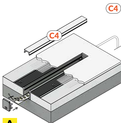
A LED profile HIDE10 C4 profil LED HIDE10 C4
