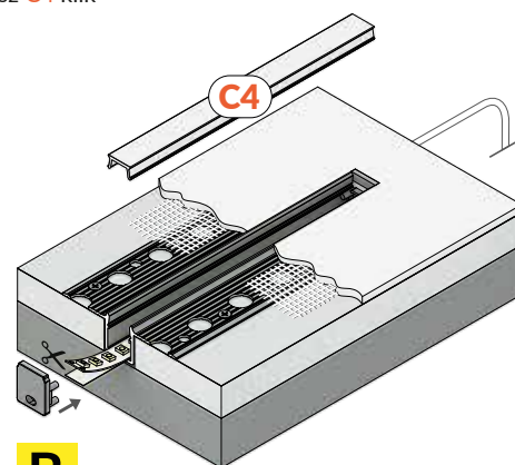
B LED profile HIDE10 C4 PLUS profil LED HIDE10 C4 PLUS
